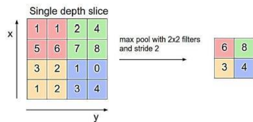
Gambar 7. Operasi Max Pooling [6]
