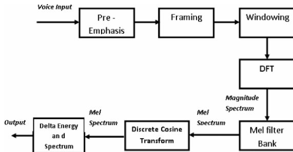
Gambar 2. Proses Perhitungan MFCC [4]
